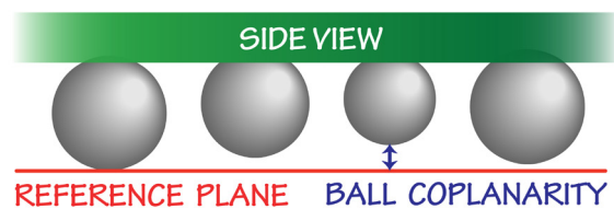
Figure 4 Ball Coplanarity
