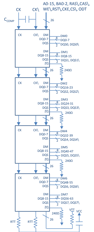
Figure 3: Functional Block Diagram
