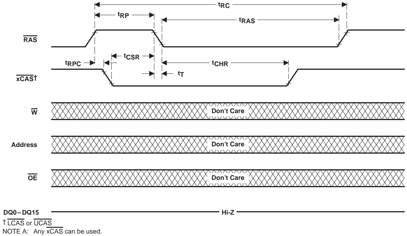
Figure 11. Automatic-xCBR-Refresh-Cycle Timing
