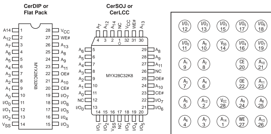
Figure 1 - Pin Configuration
