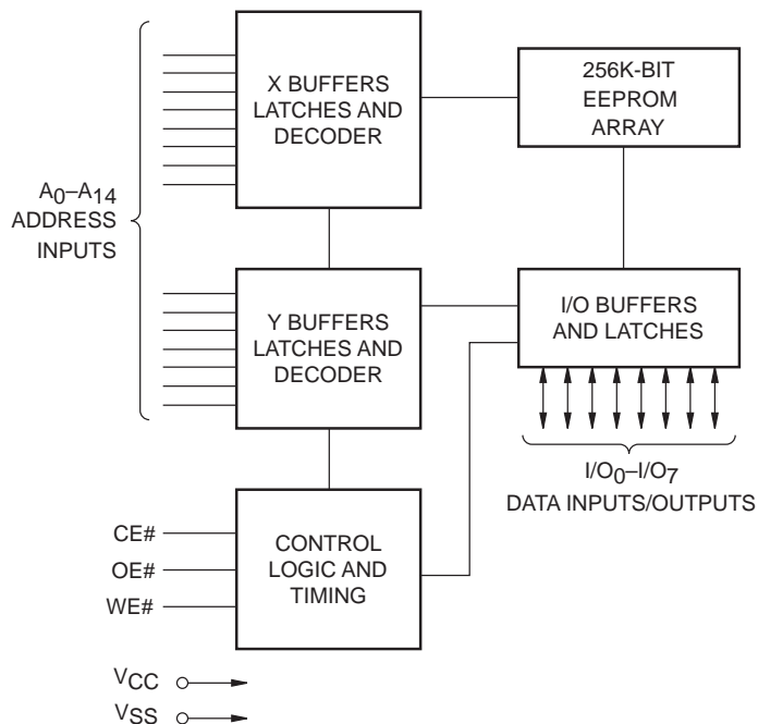
Figure 2 - Functional Diagram
