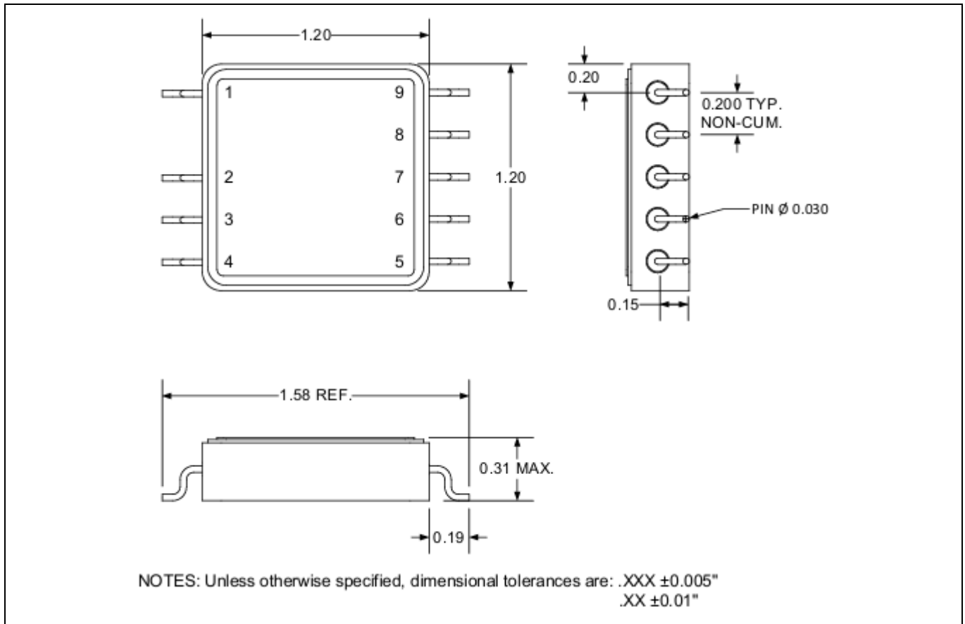
Figure 9 Package outline
