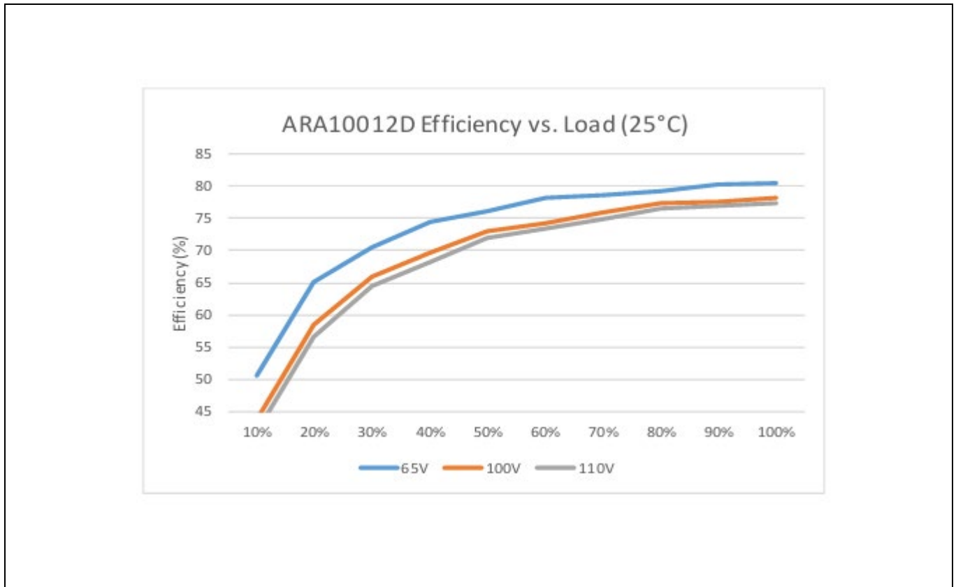
Figure 5 ARA10012D Efficiency vs. Load (25°C)
