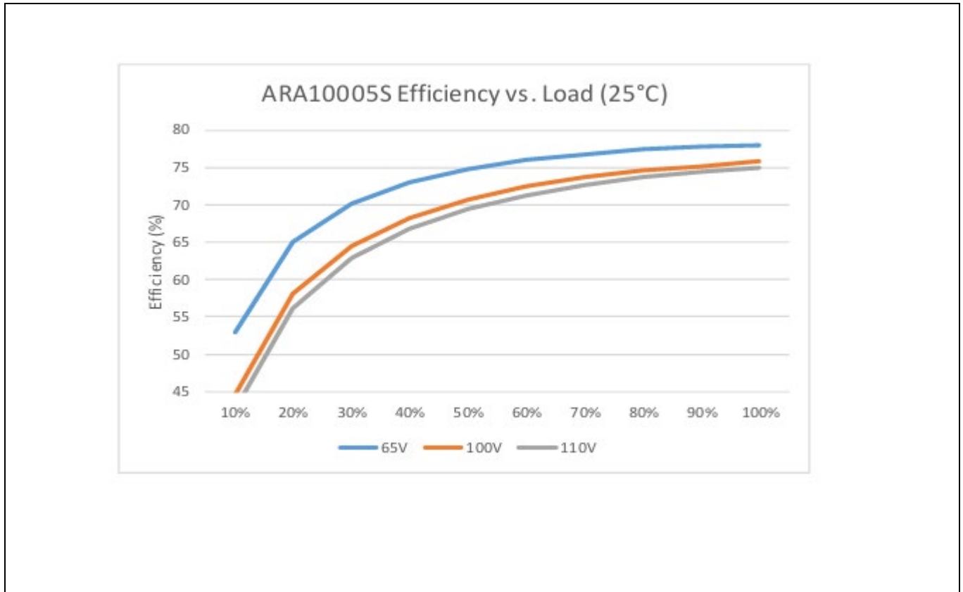
Figure 3 ARA10005S Efficiency vs. Load (25°C)
