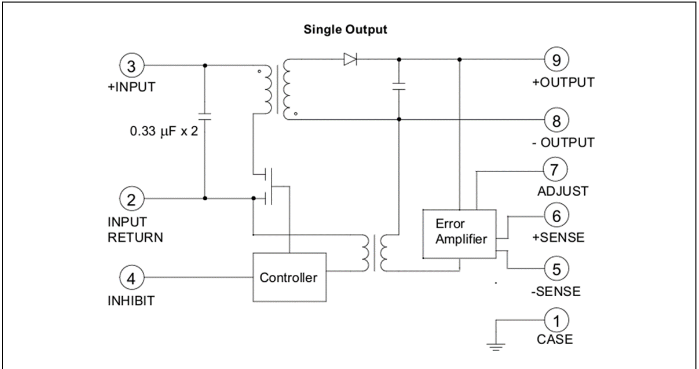
Figure 1 Block Diagram - Single Output
