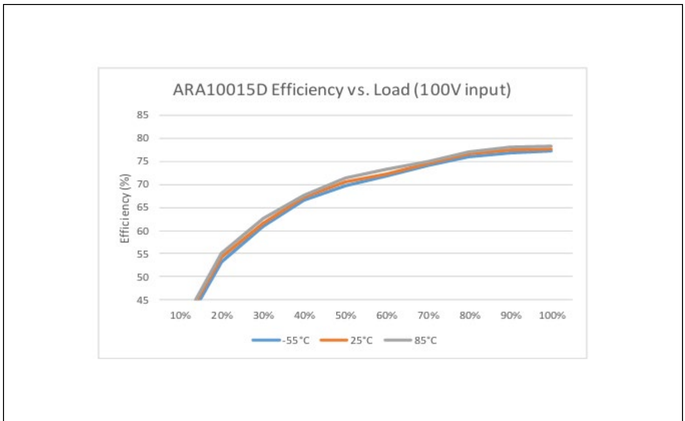
Figure 8 ARA10015D Efficiency vs. Load (100V input)
