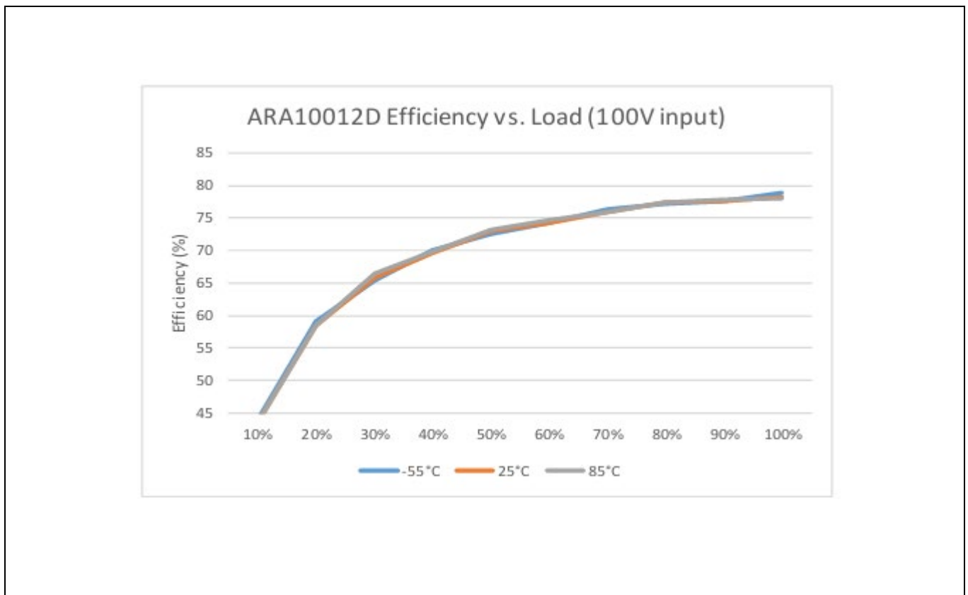
Figure 6 ARA10012D Efficiency vs. Load (100V input)
