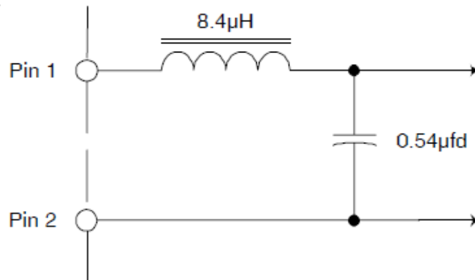
Figure 4. Input Filter Circuit
