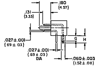
Arrangement for Sizes 7, 17 & 23
