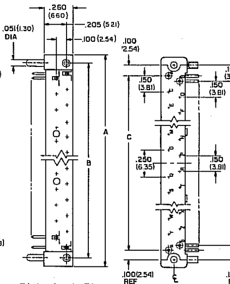
Right-Angle Pins
