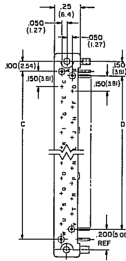
Arrangement for Sizes 7, 17 & 23
