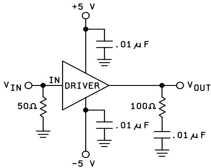
AC test circuit
