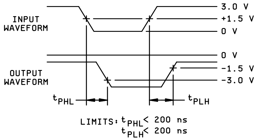
AC waveforms
