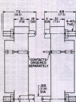
Socket Contacts (Shown with guide hardware) Pin Contacts (Shown with guide hardware)
