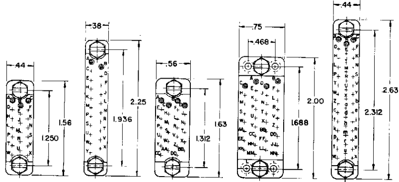
20 - 20PSK 21 - 20PSK 26 - 20PSK 34 - 20PSK 41 - 20PSK 20 - 20SS 21 - 20SS 26 - 20SS 34 - 20SS 41 - 20SS
