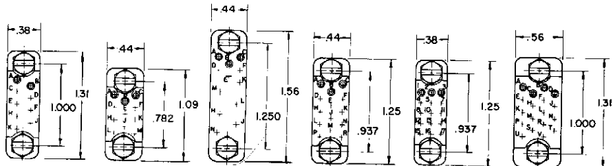
9 - 20PSK 11 - 20FSK 12-20PSK 14 - 20PSK 15-20PSK 18 - 20PSK 9 - 20SS 11 - 20SS 12-20SS 14 - 20SS 15-20SS 18 - 20SS
