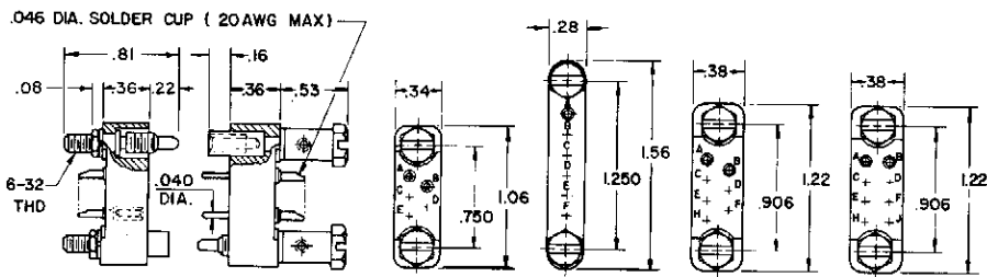
RECEPTACLE PLUG 5 - 20PSK 6 - 20PSK 7 - 20PSK M8 - 20PSK 5 - 20SS 6 - 20SS 7 - 20SS M8 - 20SS
