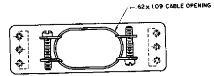
50 - 20H2 LARGE CABLE OPENING 50 - 20H00 NO CABLE OPENING
