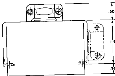
42 - 20H (TOP CABLE OPENING .58 x .75) 42 - 20H - 1 (SIDE CABLE OPENING .44 x .59)
